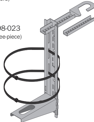
Hook the suspension beam of the 3-pc. model to the water heater nipple to support tanks vertically against the side wall of the heater tank. (Use extension piece for larger heaters)
